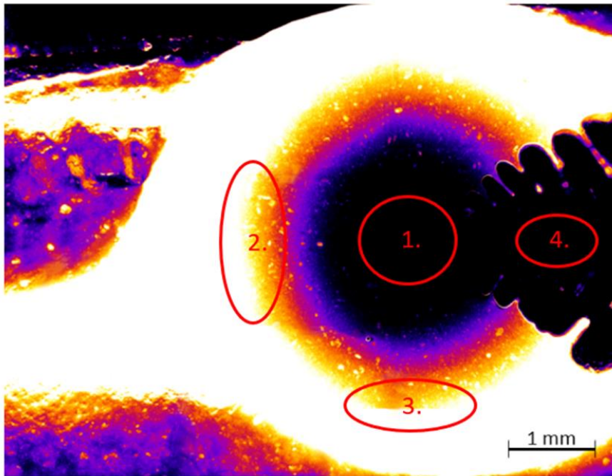
Fluorescence contact ball-on-disc
