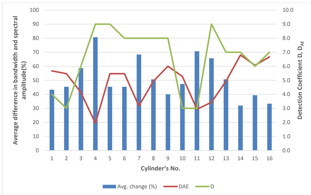
Figure 6.7 Rate changes caused by that damage coefficient and Deflection (DAE).
