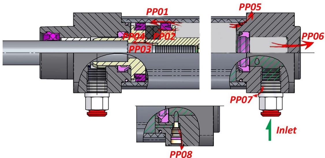
Figure 5.6 Leaks below the piston in the progress stroke [53].
