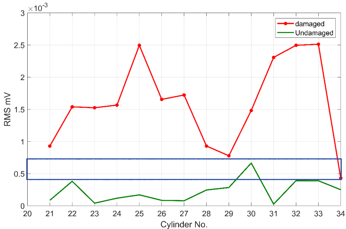
Figure 6.23 Comparing between damaged and undamaged cylinders NP08, PP03, NP07
