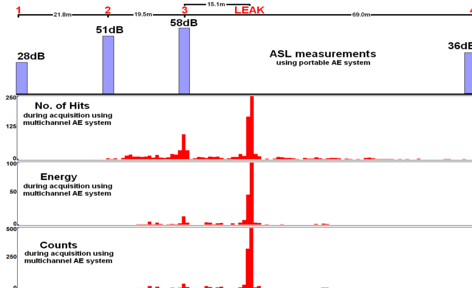
Figure 2.5 ASL vs. channel (top) and linear location indicating the leak point based on number of hits, energy and counts (bottom) of the acquired signals, after only 240 seconds of acquisition [48].
