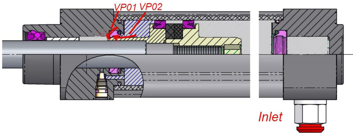
Figure 5.7 Leaks during damping in progress stroke [53].
