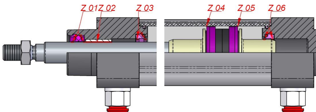
Figure 5.9 Places of galling [53].
