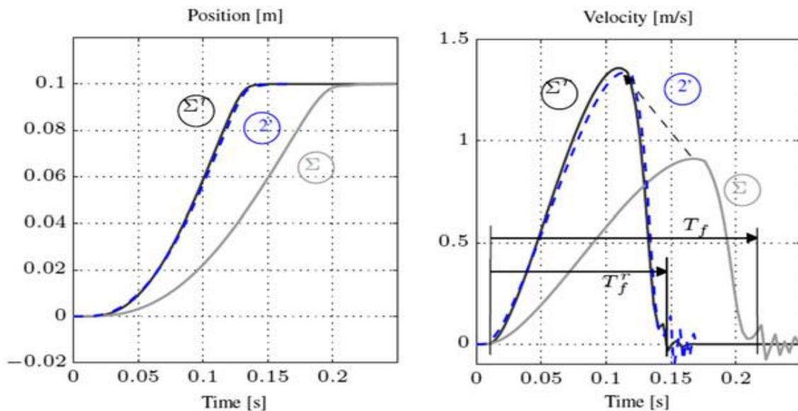
Figure 2.7 Illustration of a similar system dynamics between two systems [52].
