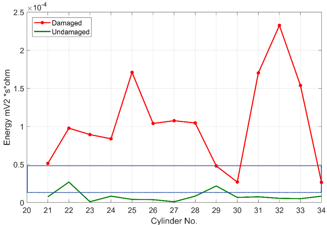
Figure 6.20 Comparing between damaged and undamaged cylinders by Energy.
