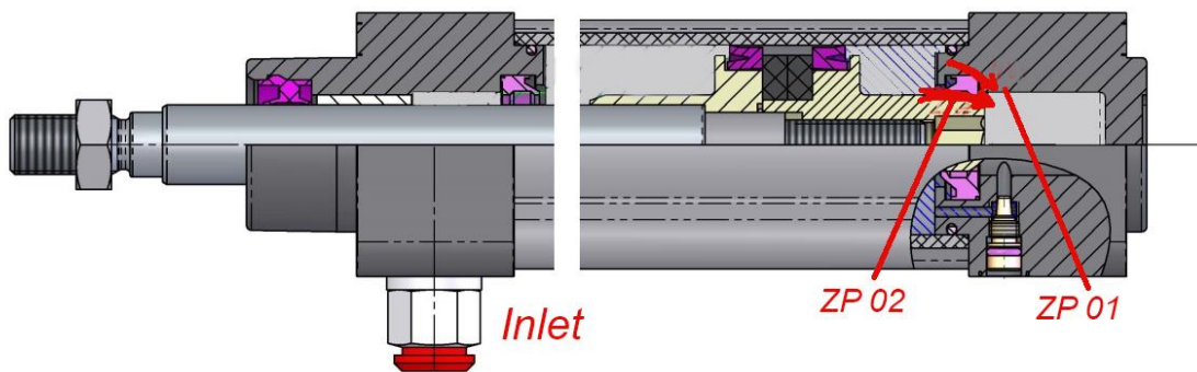
Figure 5.8 Leaks during damping in retreat stroke [53].
