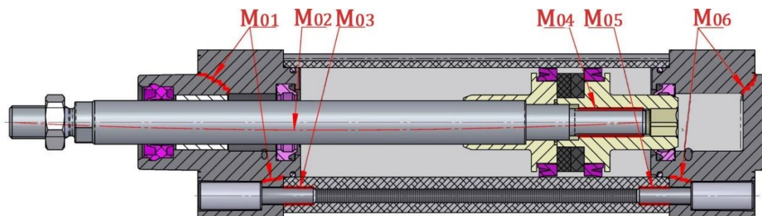
Figure 5.10 Mechanical defects [53].
