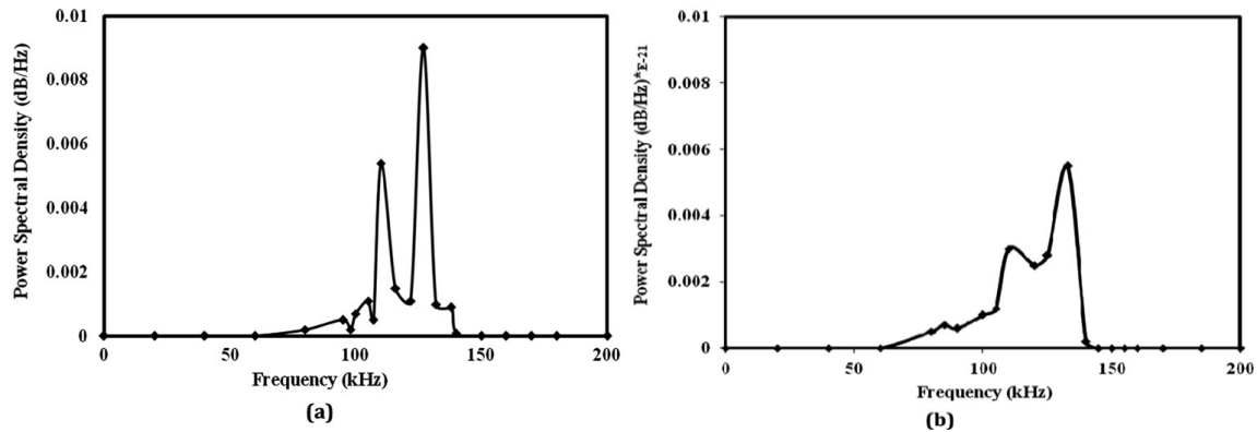
Figure 2.4 FFT results of test no. 1 for sensor S1 (a) experimental, (b) theoretical [47].
