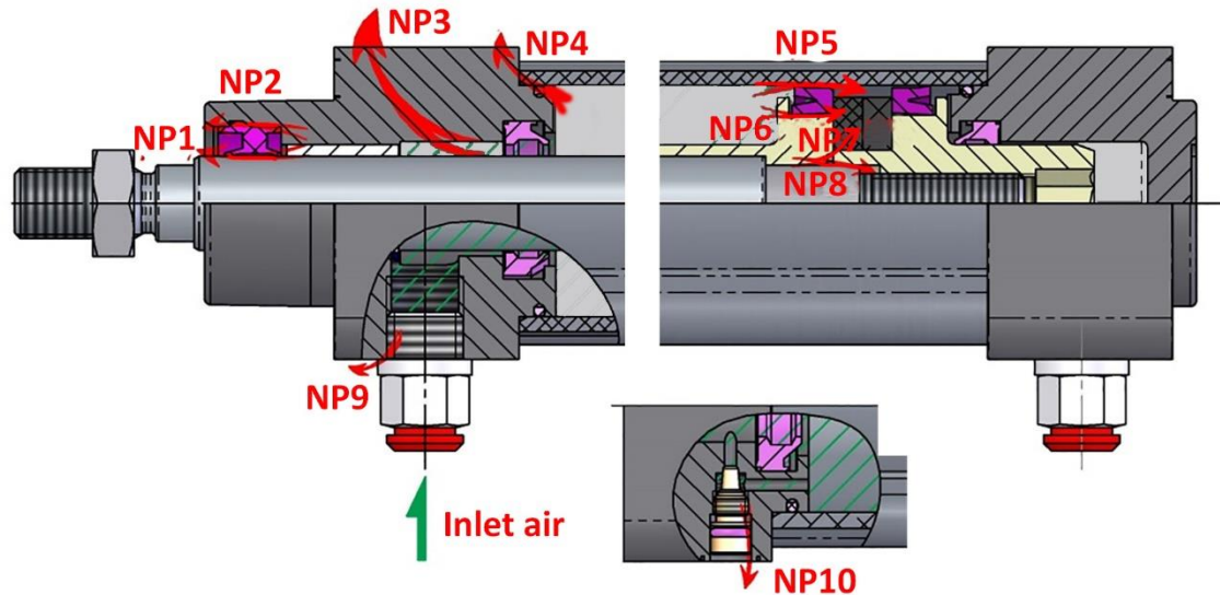
Figure 5.5 Leaks above the piston in the retreat stroke [53].
