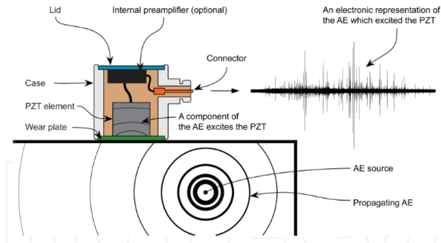
Figure 5.15 Illustration of a typical resonant piezoelectric AE transducer and how an AE is converted into an electric representation [54].
