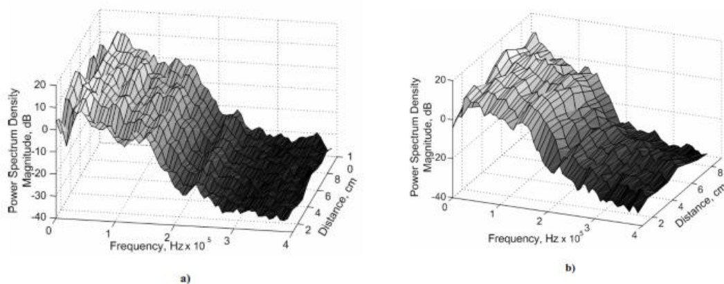
Figure 2.6 Power spectrum densities of the HFV at various measurement points: a) new pneumatic cylinder; b) worn pneumatic cylinder [50].
