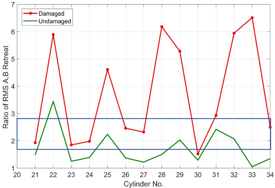
Figure 6.19 Comparing between damaged and undamaged cylinders by ratio of RMS.
